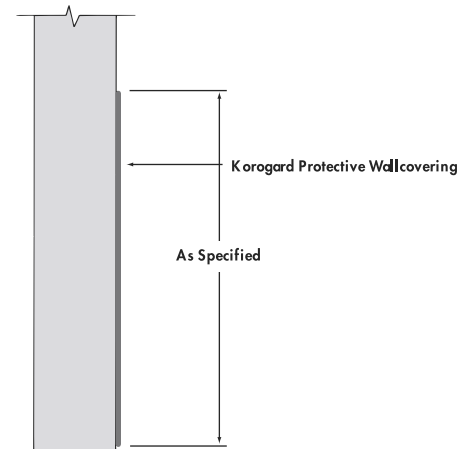
Kickplate/Pushplate
