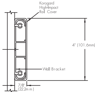
Model C460
