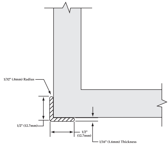
Anodized Aluminum Corner Guards
